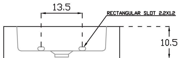
Front Elevation
