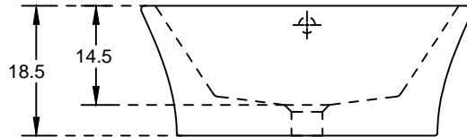
FRONT ELEVATION
