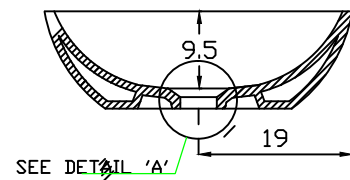
SECTIONAL VIEW
