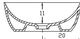
Sectional View
