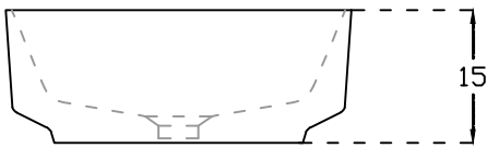
FRONT ELEVATION
