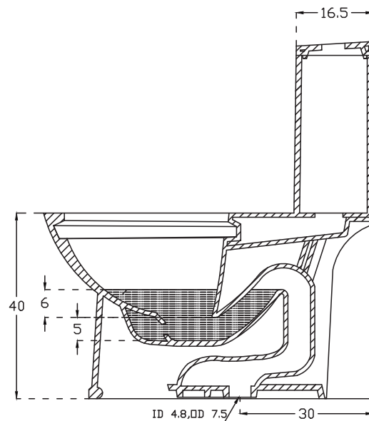
Sectional View
