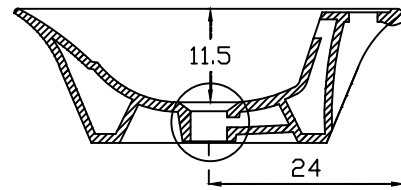
SECTIONAL VIEW
