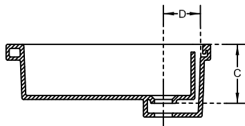
SECTIONAL VIEW
